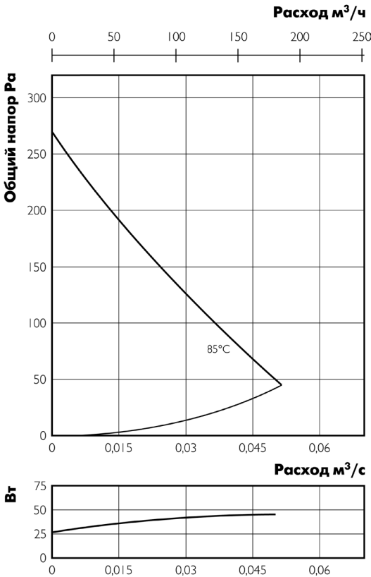
RS 125 A
