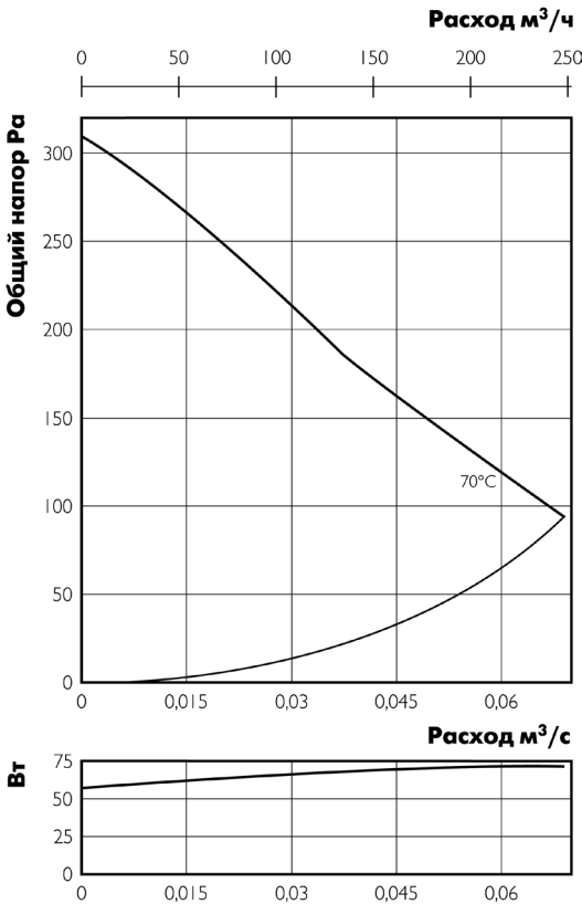
RS 125 C
